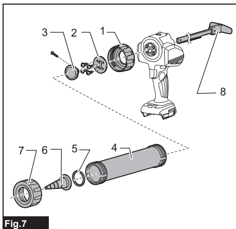
► 1. Joint de support 2. Plaque 3. Piston 4. Support 5. Anneau de caoutchouc 6. Buse 7. Joint de support (comme capuchon) 8. Tige
